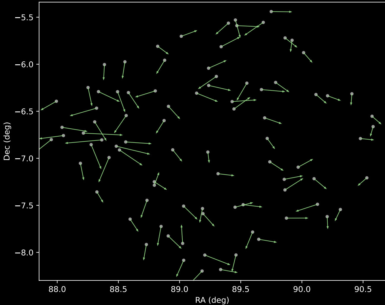
APOGEE DR17 Cluster 5 Proper Motion Vectors (n=87)
