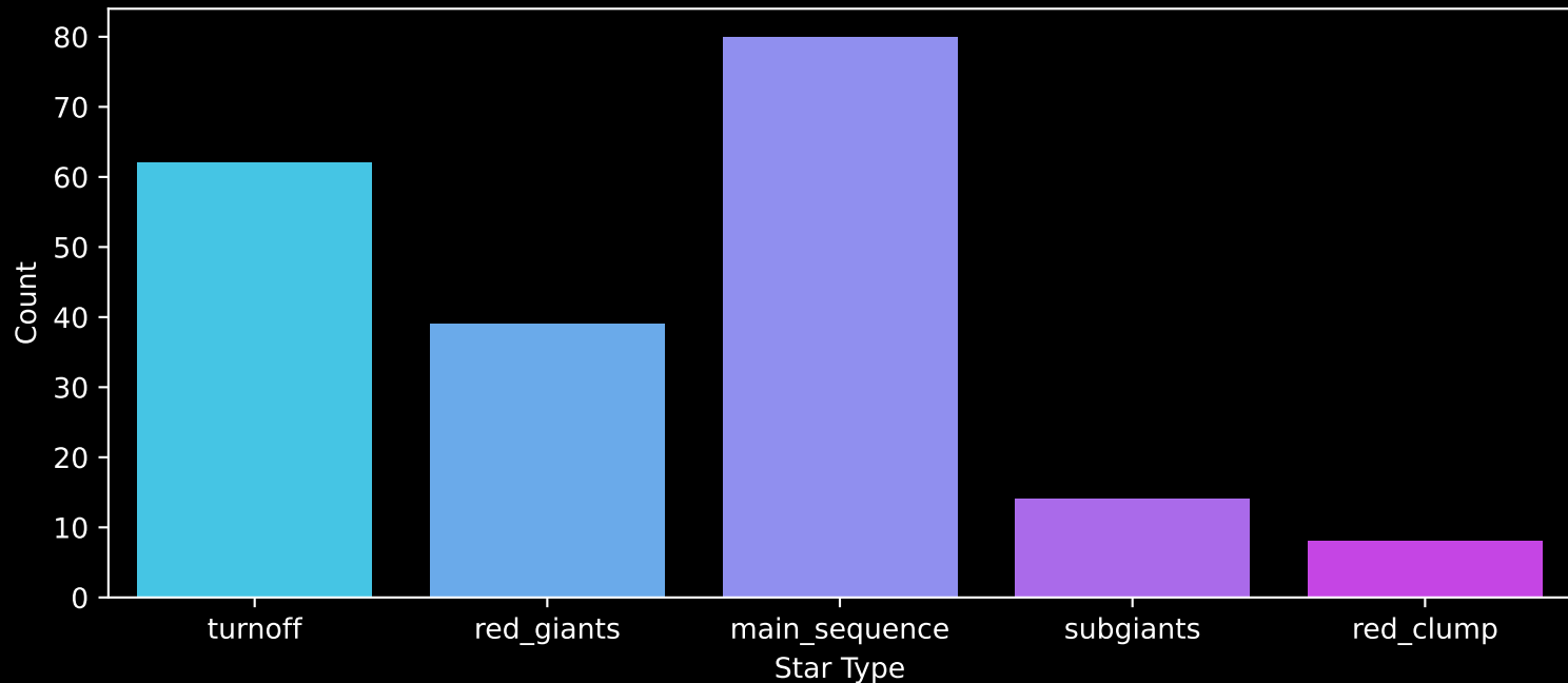
APOGEE DR17 Field: [K2_C12_071-60_btx] Count plot of Star Type
