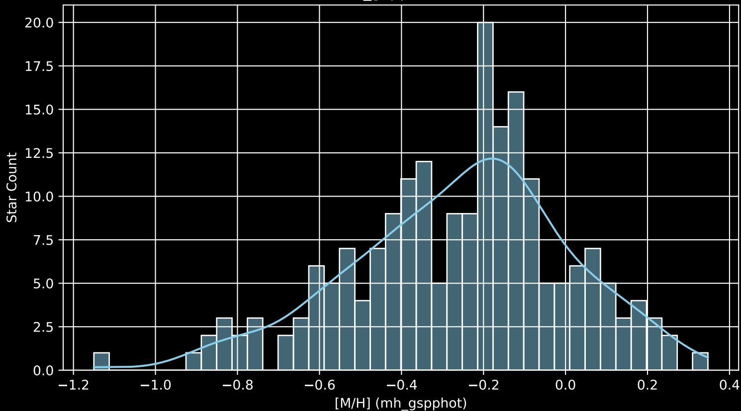
APOGEE DR17 Field: [K2_C12_071-60_btx [M/H] (mh_gspphot) (n= 203)
