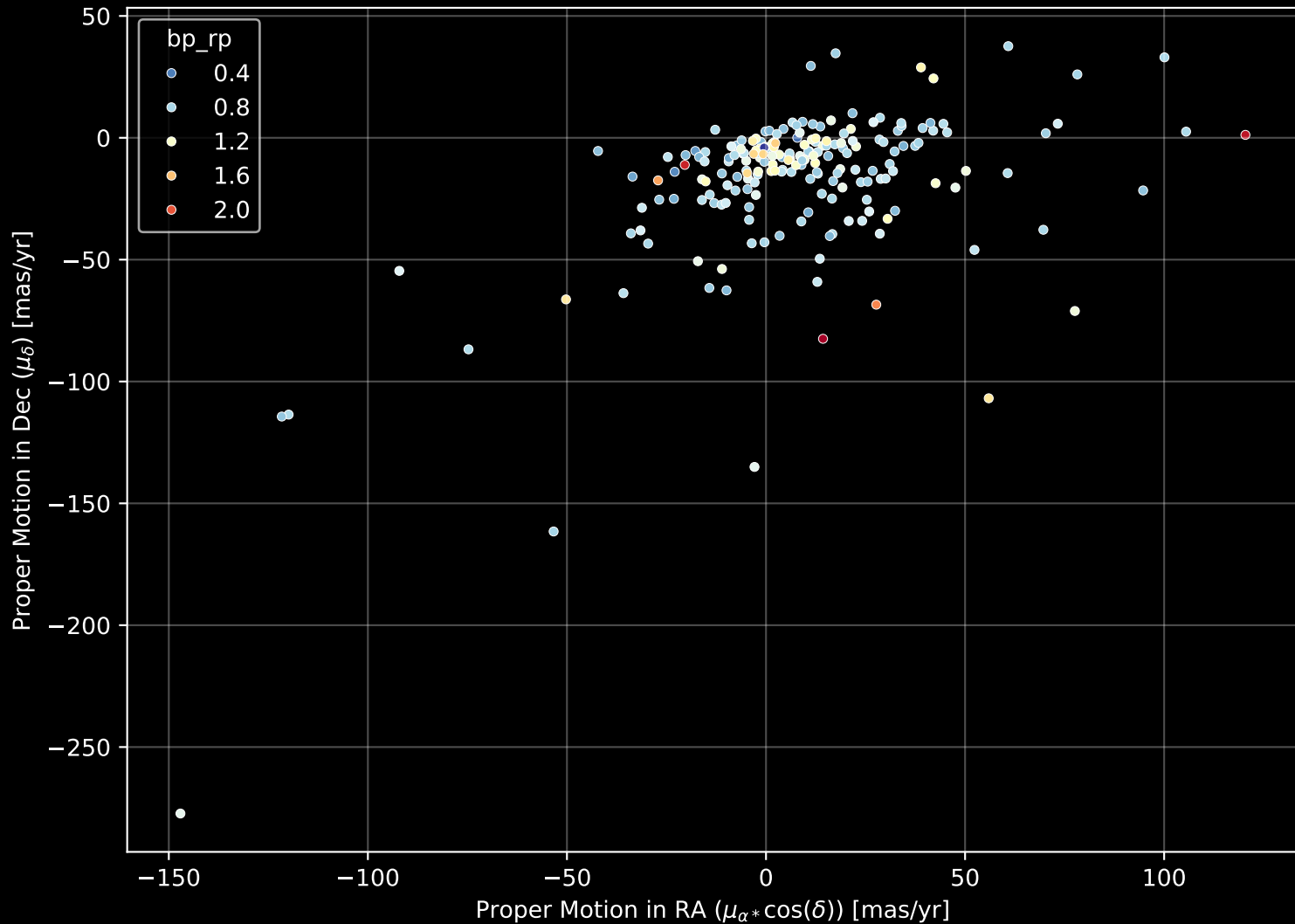
APOGEE DR17 Field: [K2_C12_071-60_btx] Proper Motion Diagram (n= 203)
