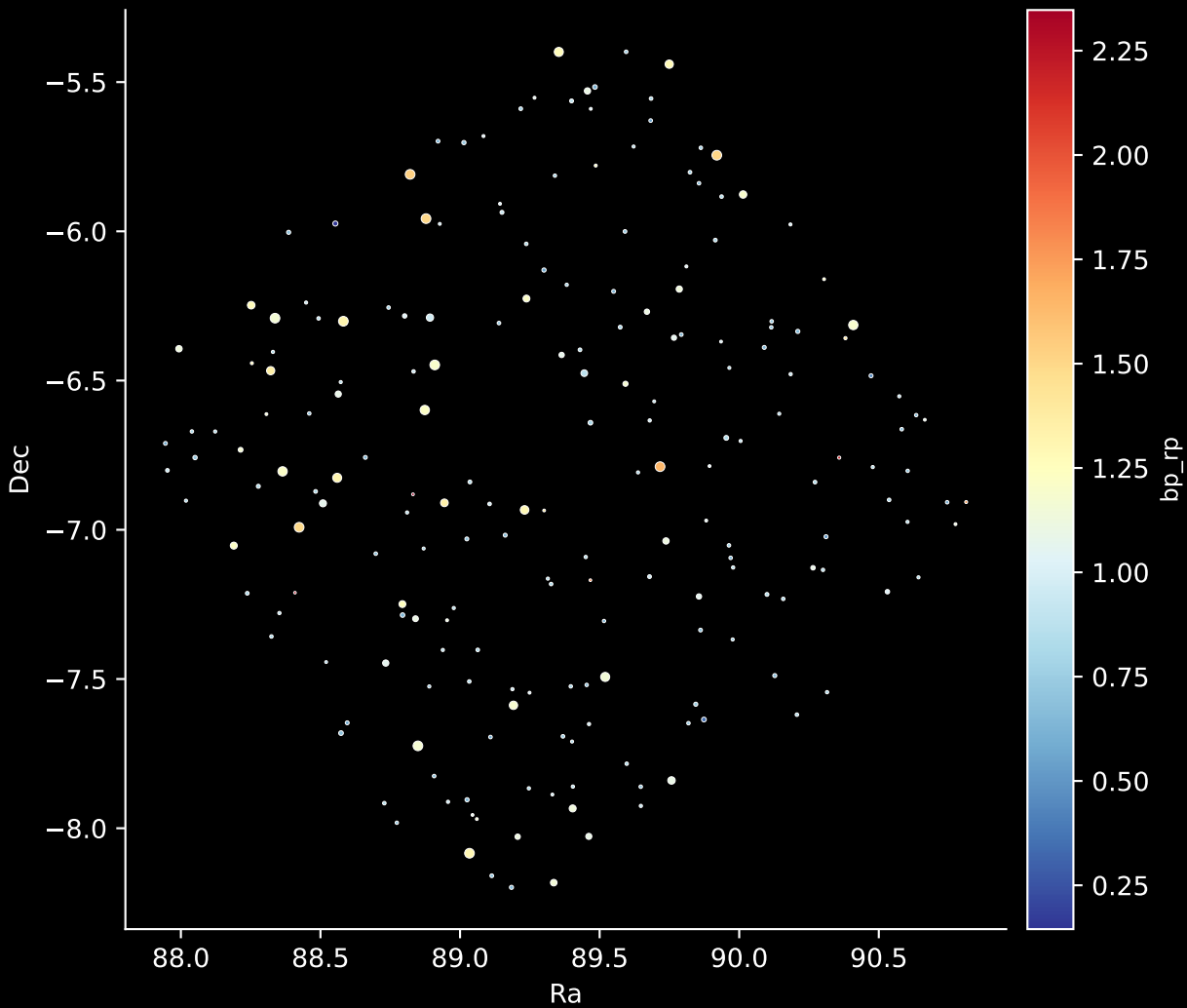
APOGEE DR17 Field: [K2_C12_071-60_btx] Stars: 203
