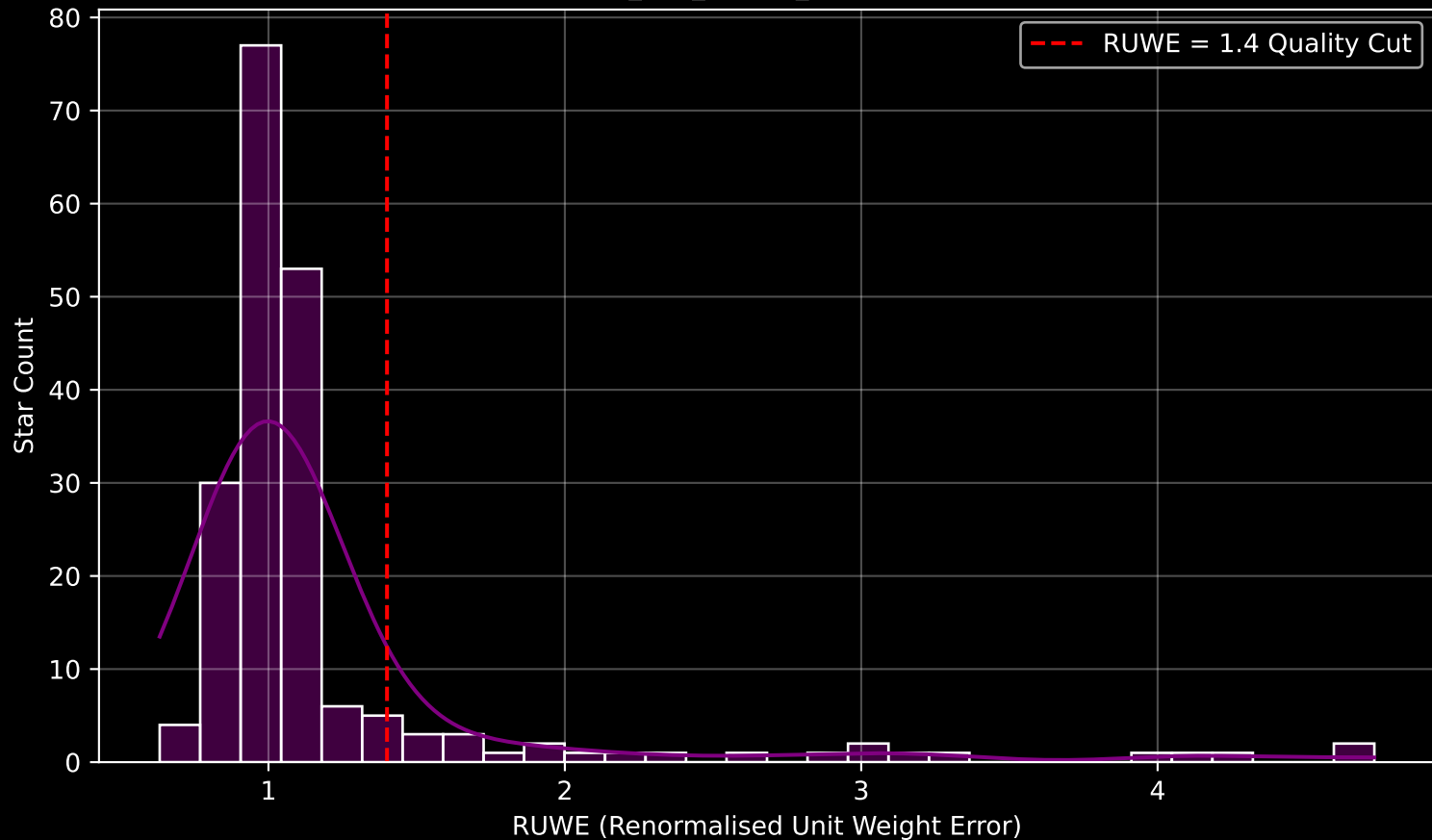
GAPOGEE DR17 Field [K2_C12_071-60_btx] RUWE Distribution (n= 198)
