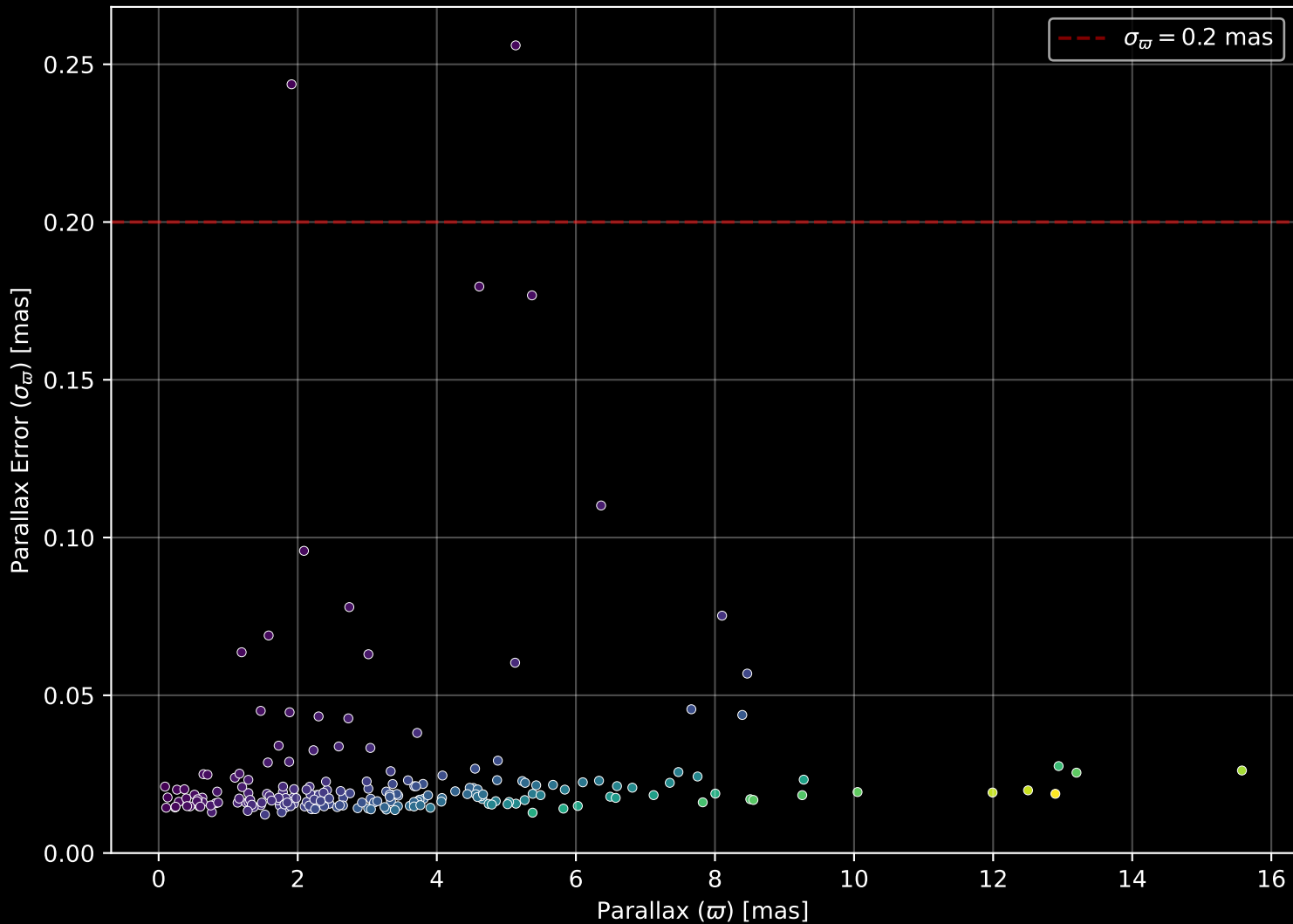
APOGEE DR17 Field: [K2_C12_071-60_btx] Parallax Quality (n= 203)
